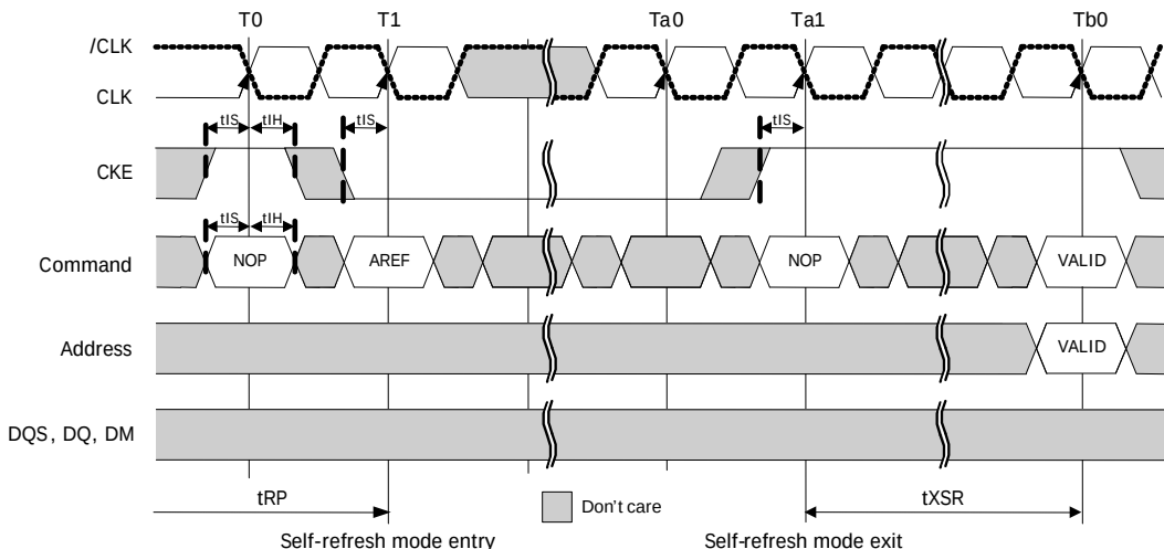
Figure 35 : Self refresh
