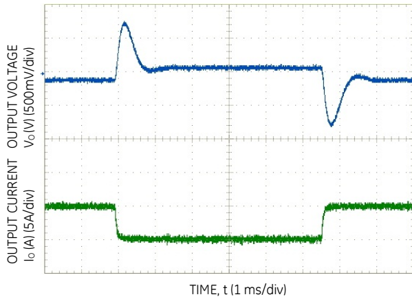
Figure 5. Typical Transient Response to Step Change in Load from 25% to 50% to 25% of Full Load at 48Vdc Input and C_o= 470\mu F Polymer, without -02 option.
