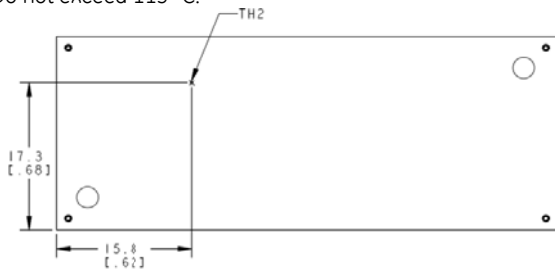
Figure 20. Location of the thermal reference temperature TH 2 for Baseplate module. Do not exceed 110 °C.
