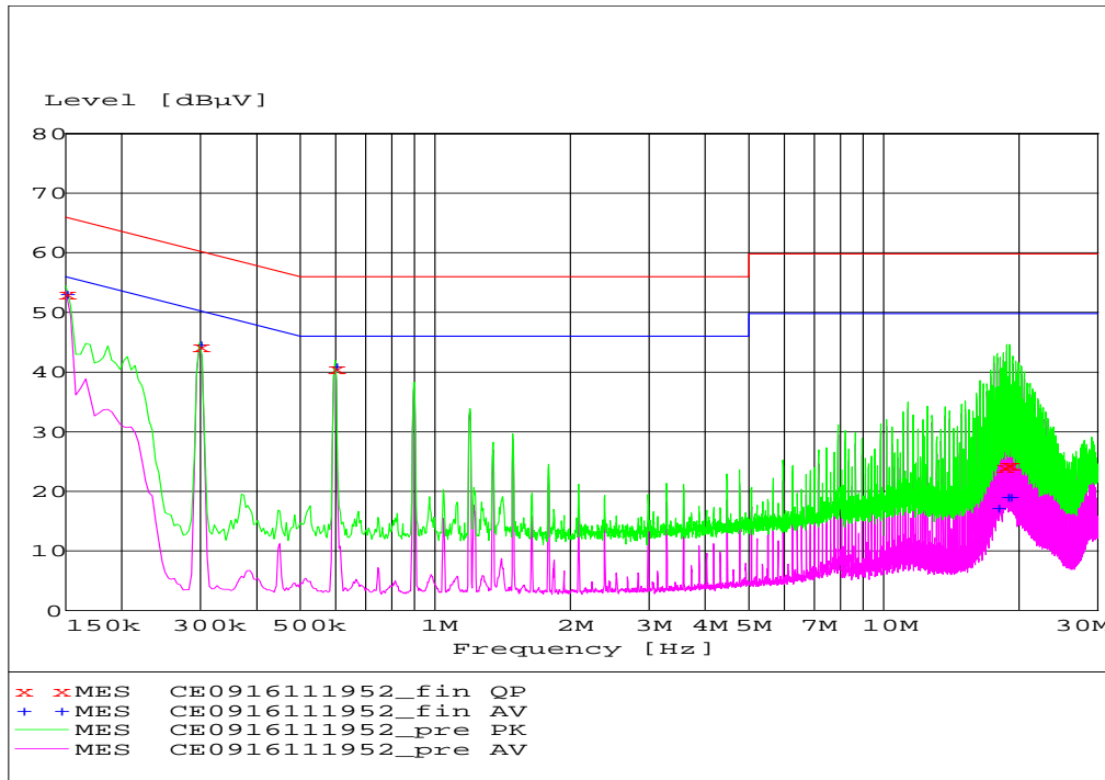
Figure 26. EMC Considerations.
