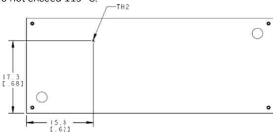
Figure 20. Location of the thermal reference temperature TH 3 for Baseplate module. Do not exceed 110 °C.
