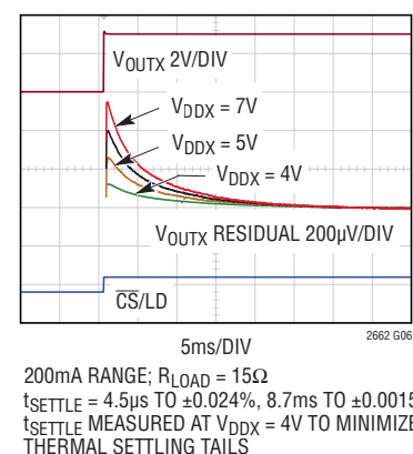
Settling 0 to 200mA Step
