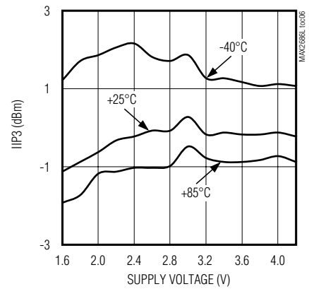
MAX2686L OUT-OF-BAND IIP3 vs. SUPPLY VOLTAGE AND TEMPERATURE (TONE 1 AT 1713MHz, -27dBm; TONE 2 AT 1851MHz, -39dBm)
