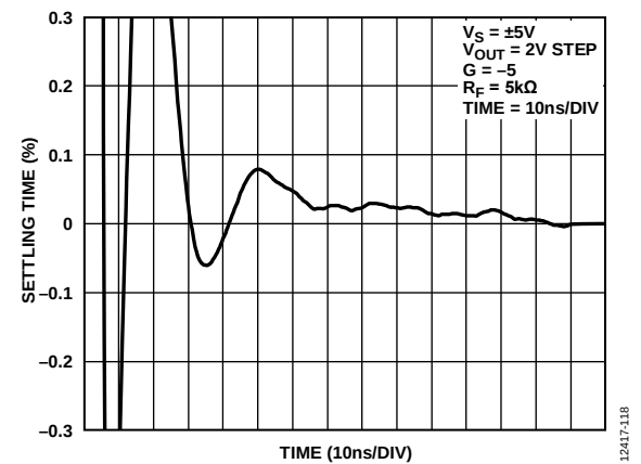
Figure 20. 0.1% Settling Time
