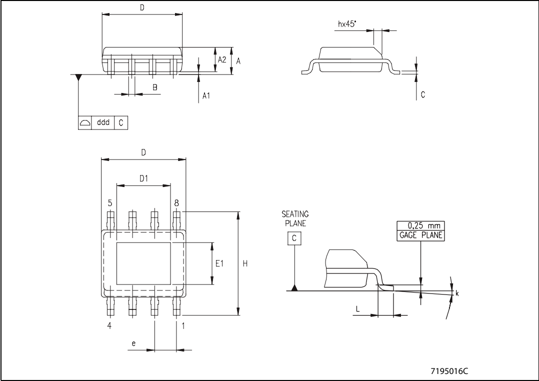
Figure 40. Package dimensions
