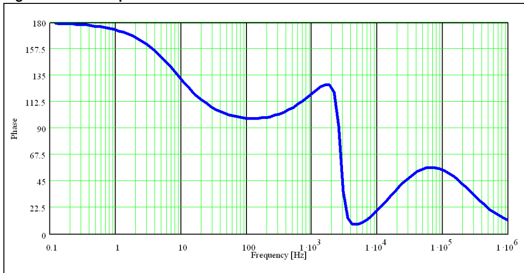
Figure 12. Phase plot
