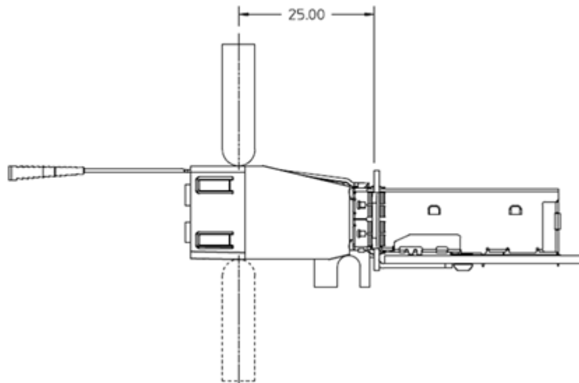
Figure 1: Longitudinal Loading
