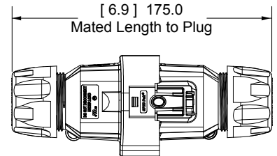
Mated View
