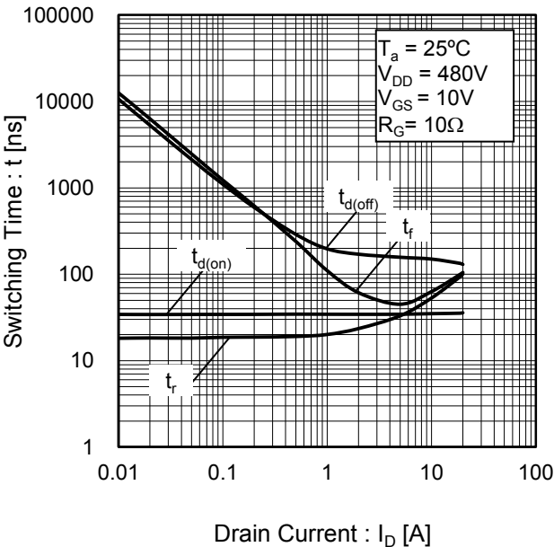
Fig.19 Switching Characteristics
