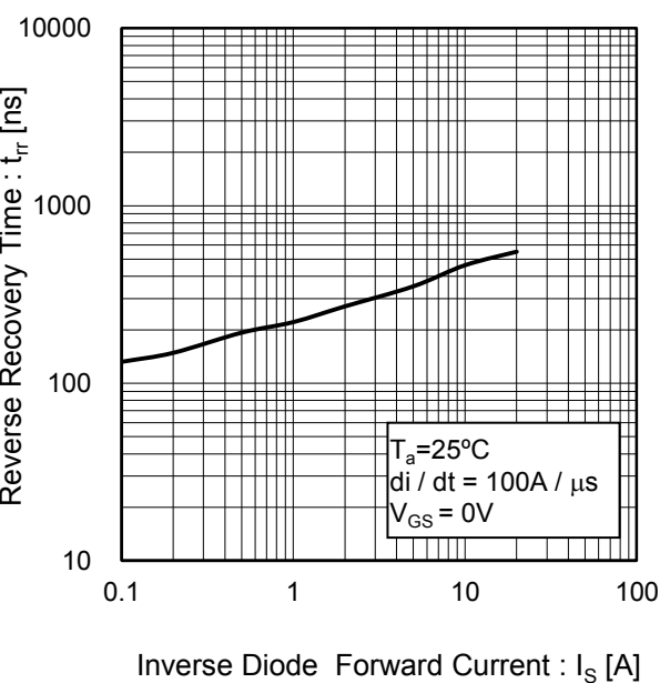
Fig.22 Reverse Recovery Time vs. Inverse Diode Forward Current
