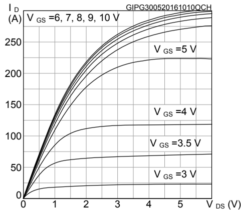
Figure 3. Output characteristics
