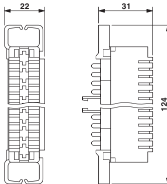
Dimensioned drawing
