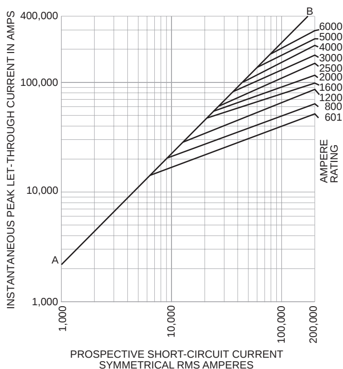
Current-Limitation Curves
