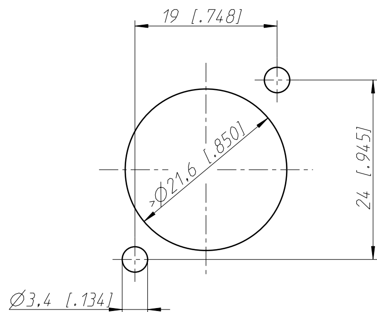
Frontplattenausschnitt (Montage von vorne) Panel cut out (Panel-mounting otion front side)
