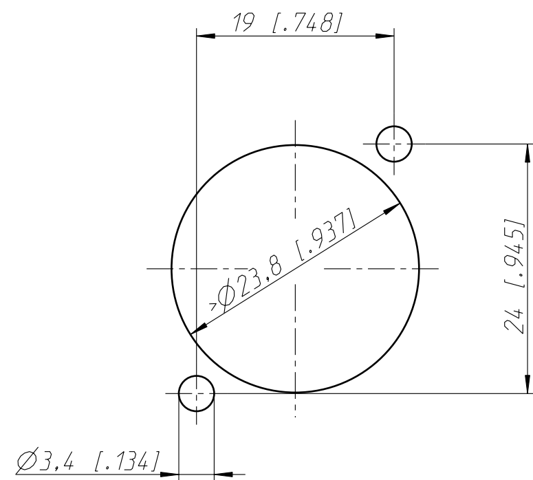
Frontplattenausschnitt (Montage von hinten) Panel cut out (Panel-mounting otion rear side)
