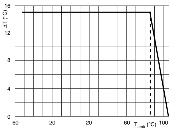
Max. allowed component temperature rise as a function of ambient temperature
