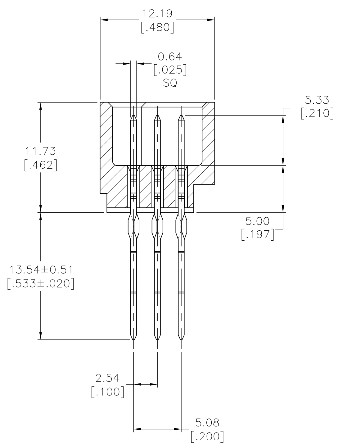
SECTION T-T
