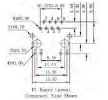
PC Board Layout Component Side Shows
