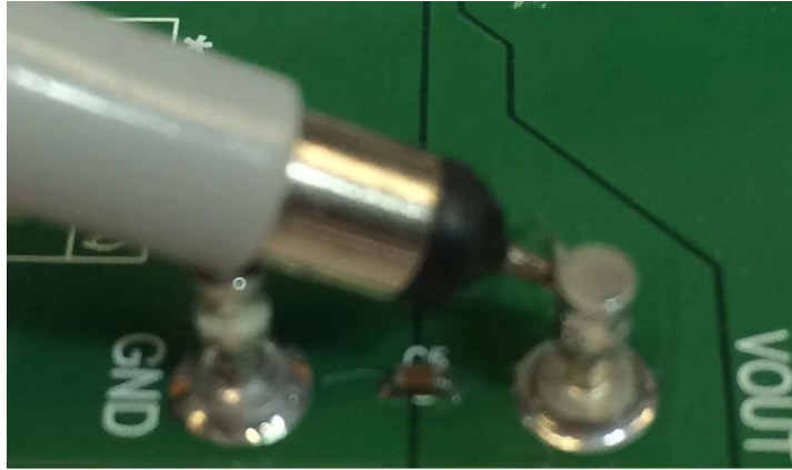
Figure 3. Output Ripple Measurement Technique
