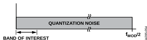
Figure 44. \Sigma\text{-}\Delta ADC Quantization Noise (Linear Scale X-Axis)
