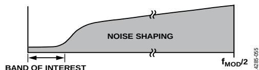
Figure 45. \Sigma\text{-}\Delta ADC Noise Shaping (Linear Scale X-Axis)
