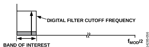
Figure 46. \Sigma\text{-}\Delta ADC Digital Filter Cutoff Frequency (Linear Scale X-Axis)
