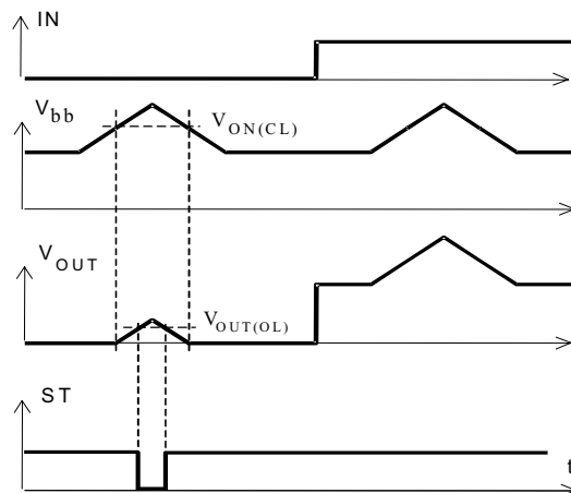
Figure 7: Overvoltage
