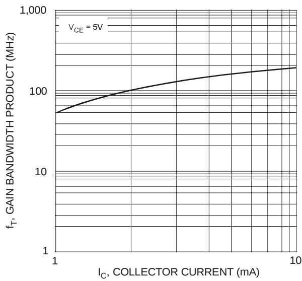
Fig. 10, Typical Gain Bandwidth Product vs. Collector Current (DRDN005W)
