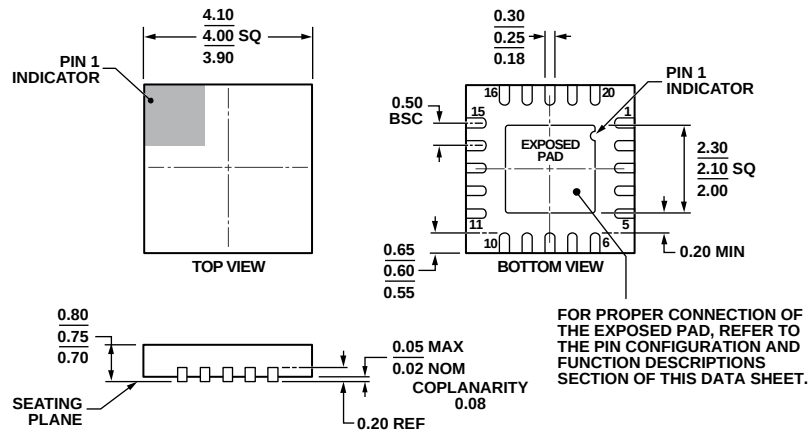
Figure 26. 20-Lead Lead Frame Chip Scale Package [LFCS_P_WQ] 4 mm × 4 mm Body, Very Very Thin Quad (CP-20-6)
