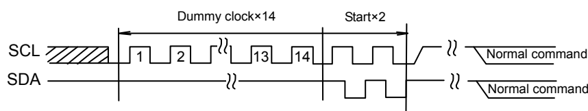
Figure 41-(a). The Case of Dummy Clock \times 14 + START + START + Command Input
