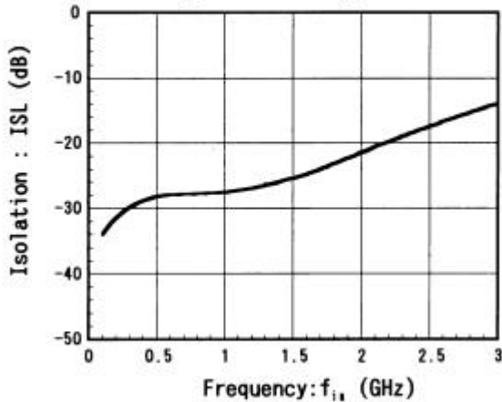
(PC-P1) Isolation vs. Frequency ( V_{CTR}=0V/2.7V , P_{is}=0dBm )
