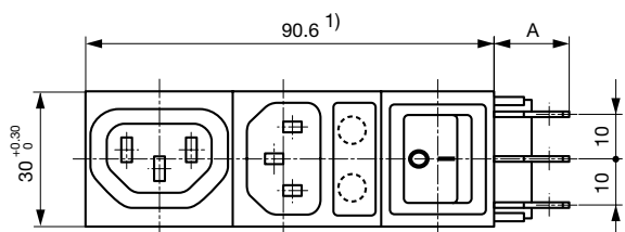
Variants 6432.0X5X.XX Mounting hole: 90.6 \pm 0.2 \times 27.6 \pm 0.2 A: Quick-connect terminal 6.3 \times 0.8 mm: 18.1 mm A: Solder terminal 3.5 \times 0.8 mm: 13.3 mm S: Panel thickness
