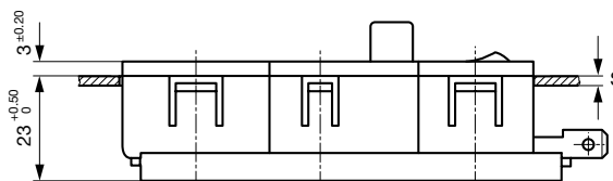
Variants 6424.0X5X.XX Mounting hole: 57 \pm 0.2 \times 27.6 \pm 0.2 A: Quick-connect terminal 6.3x0.8 mm: 18.1 mm A: Solder terminal 3.5x0.8 mm: 13.3 mm S: Panel thickness
