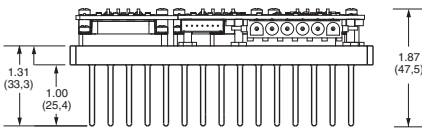
1" Fin Option Fin spacing and relief are the same for both Fin options.
