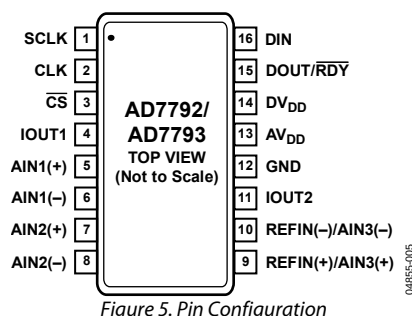
Figure 5. Pin Configuration
