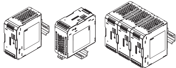
(A) Standard (Vertical) (B) Face-up mounting (C) Front, Side-by-side mounting
