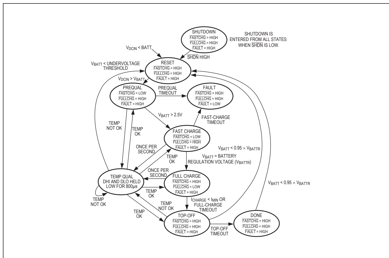
Figure 4. State Diagram
