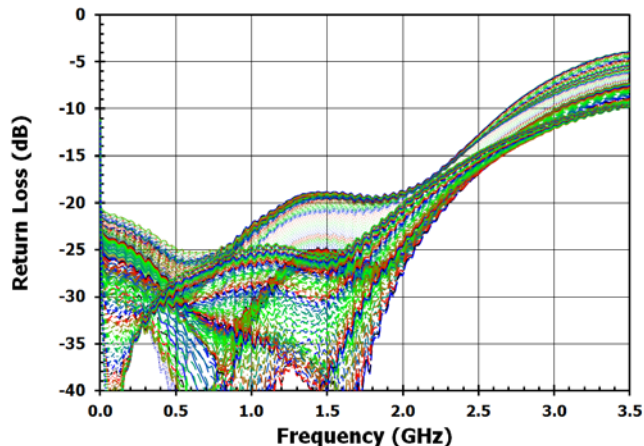
Figure 39. RF2 Return Loss vs. Frequency [ V_{\text{MODE}} = \text{LOW} ]
