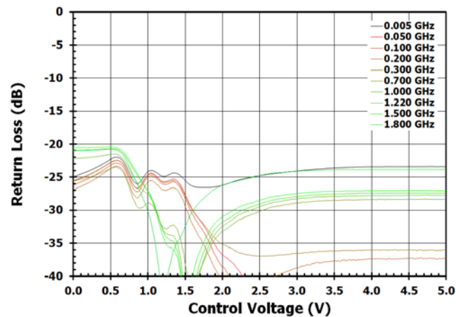
Figure 40. RF2 Return Loss vs. V_{\text{CTRL}} [ V_{\text{MODE}} = \text{LOW} ]
