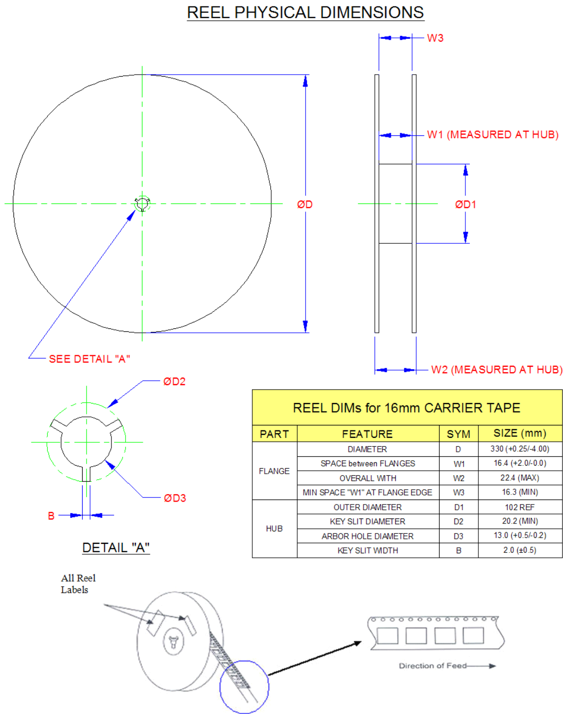
Figure 8.3 48-Pin Package Reel Specifications
