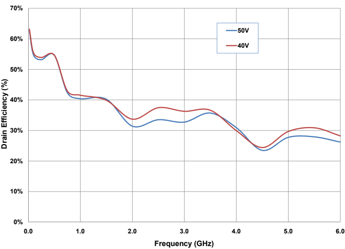
Drain Efficiency at P_{IN} = 32\text{ dBm} vs Frequency as a Function of Drain Voltage
