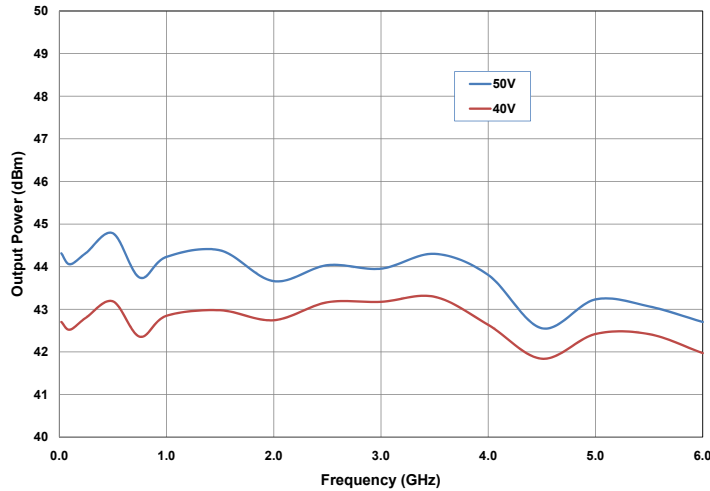
Output Power at P_{IN} = 32\text{ dBm} vs Frequency as a Function of Drain Voltage
