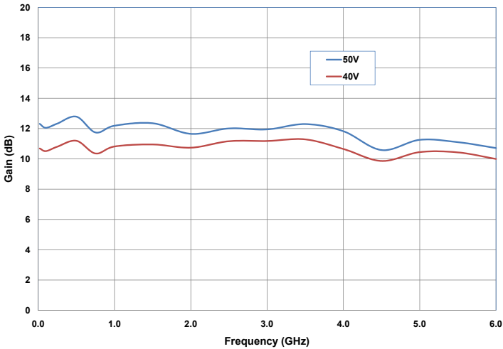
Power Gain at P_{IN} = 32\text{ dBm} vs Frequency as a Function of Drain Voltage
