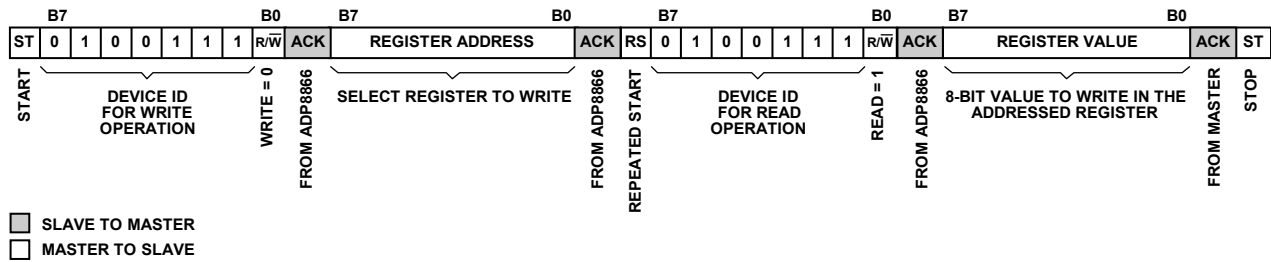
Figure 41. I 2 C Read Sequence
