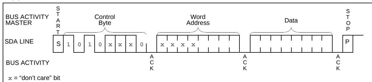
FIGURE 7-2: BYTE WRITE
