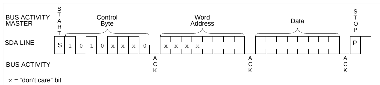
FIGURE 7-2: BYTE WRITE
