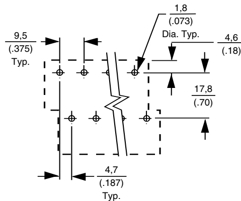
Printed Circuit Board Layout
