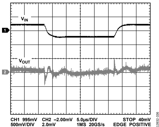
Figure 36. Line Transient Response, 500 mV Step, V_{OUT} = -1.2\text{ V} , I_{LOAD} = -500\text{ mA}
