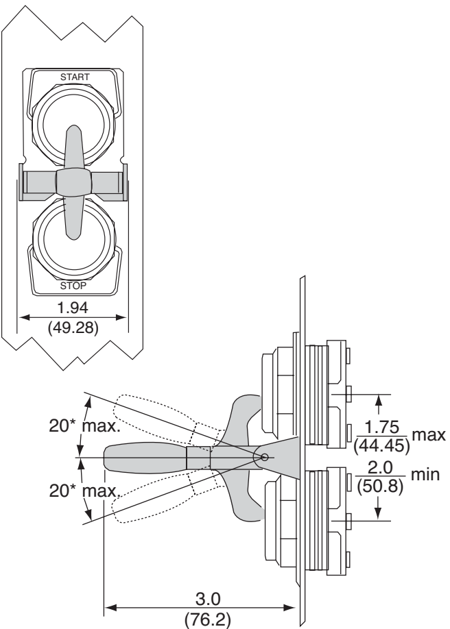
Rocker arm operating lever 9001K50
