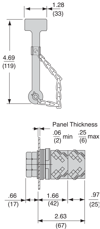
Emergency break glass operator 9001K15
