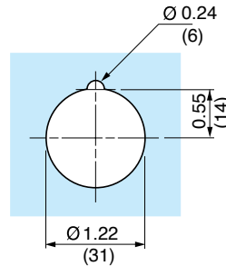
Alternate Cut-Out
