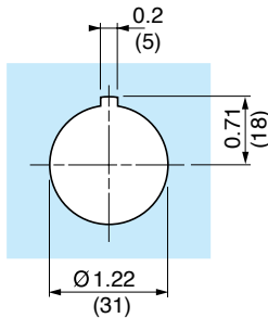
Preferred Cut-Out
