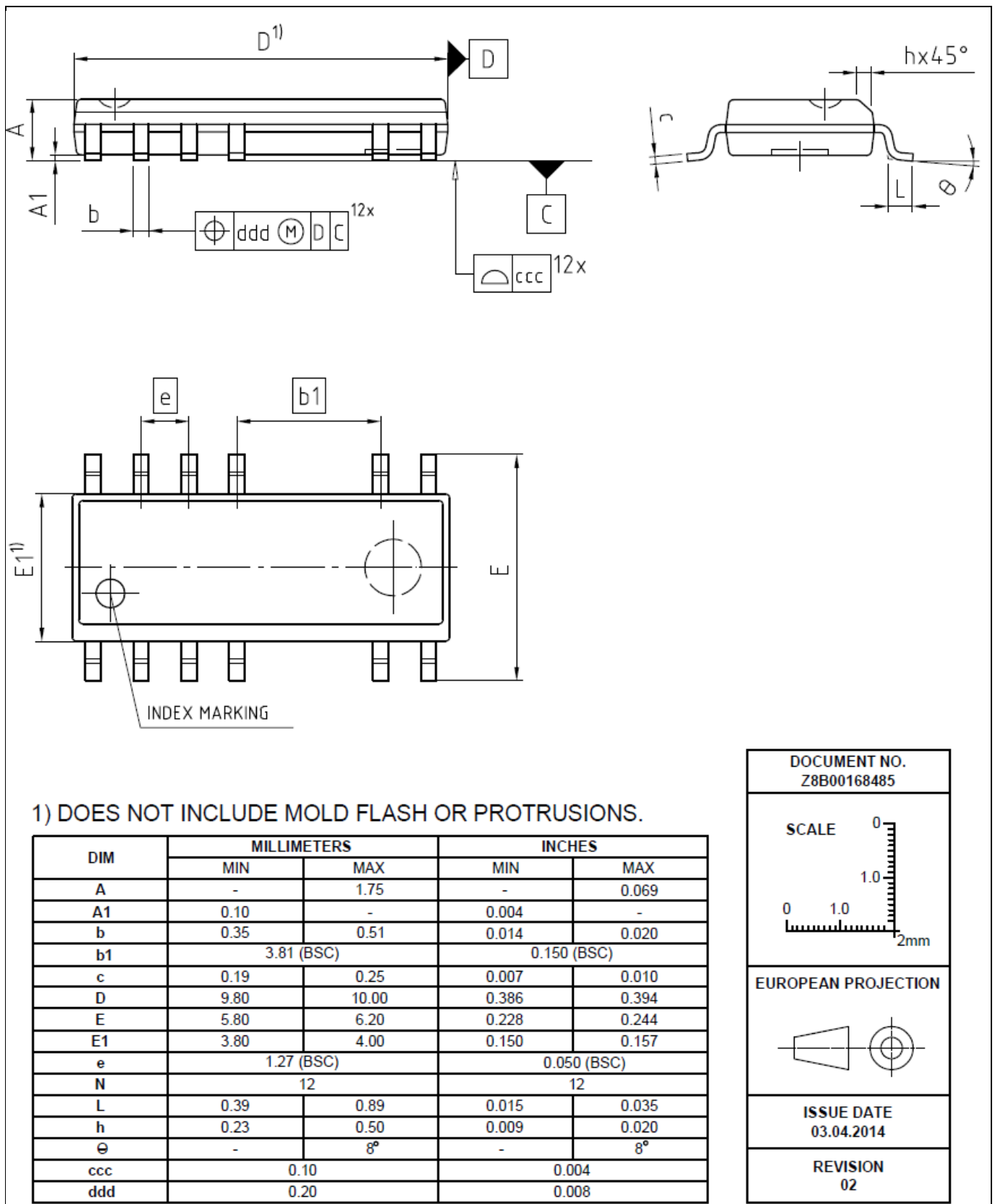
Figure 60 PG-DSO-12
