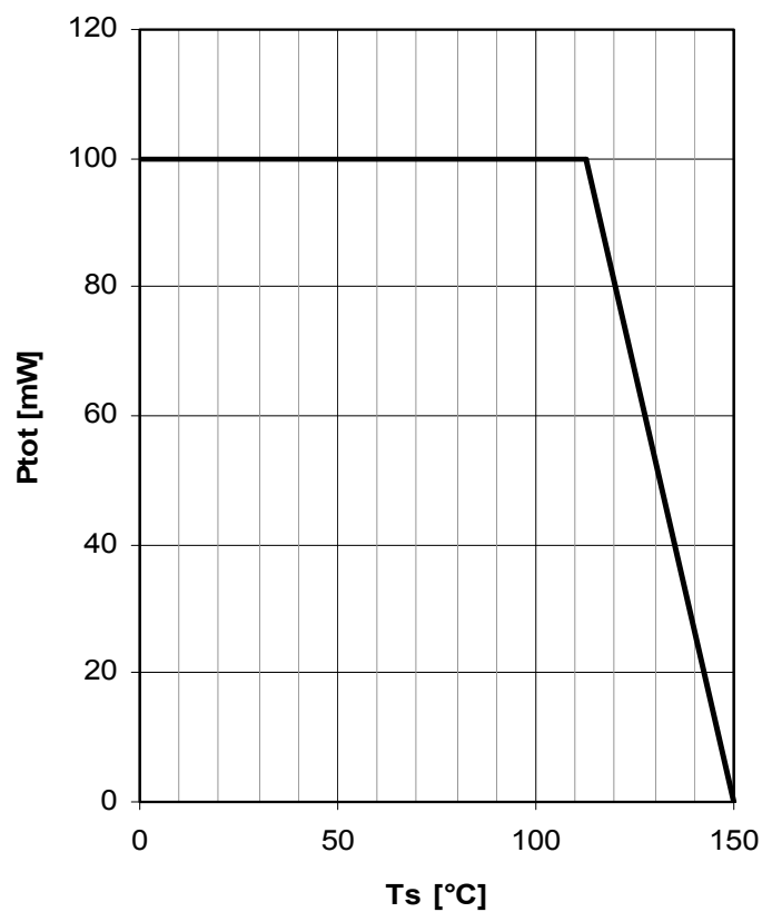
Figure 3 Total Power Dissipation P_{tot} = f(T_s)
