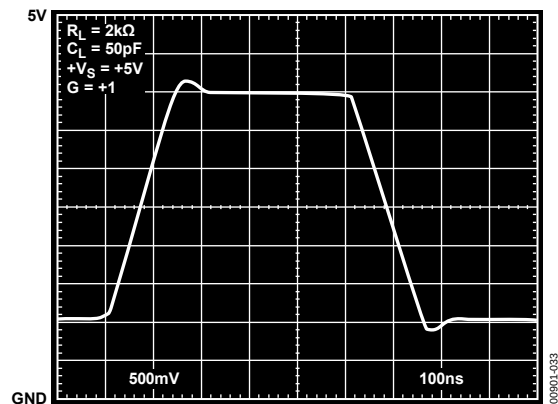
Figure 33. Pulse Response, +V_S = +5\text{ V} , G = +1
