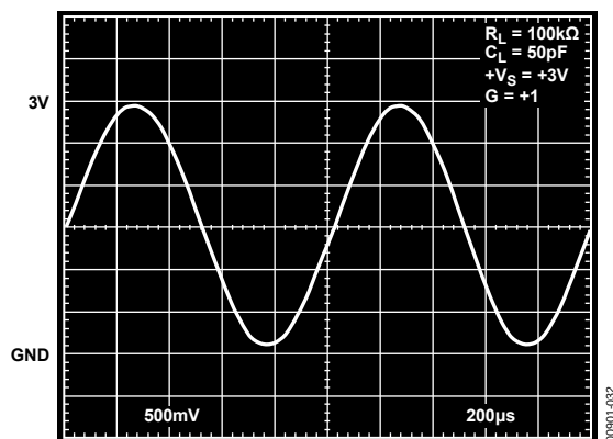
Figure 32. Output Swing, +V_S = +3\text{ V} , G = +1
