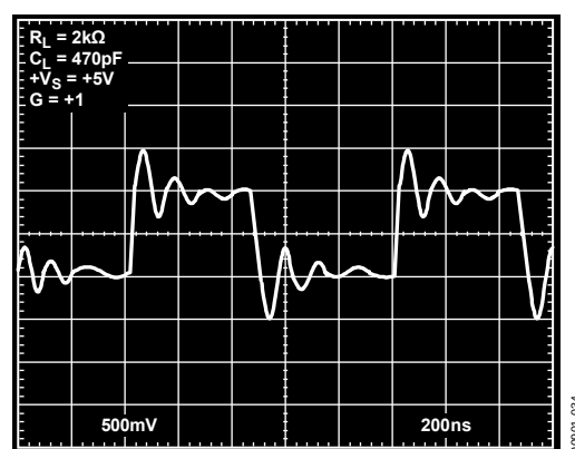
Figure 34. Pulse Response, +V_S = +5\text{ V} , G = +1 , C_L = 470\text{ pF}
