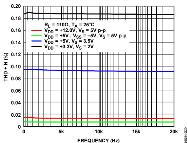
Figure 20. THD + N vs. Frequency, \pm 5 V Dual Supply
