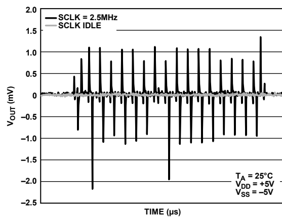
Figure 26. Digital Feedthrough
