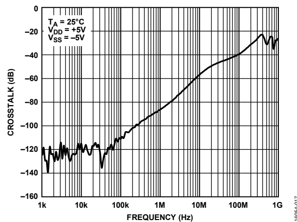
Figure 17. Crosstalk vs. Frequency, \pm 5 V Dual Supply
