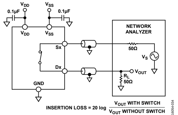
Figure 34. Bandwidth
