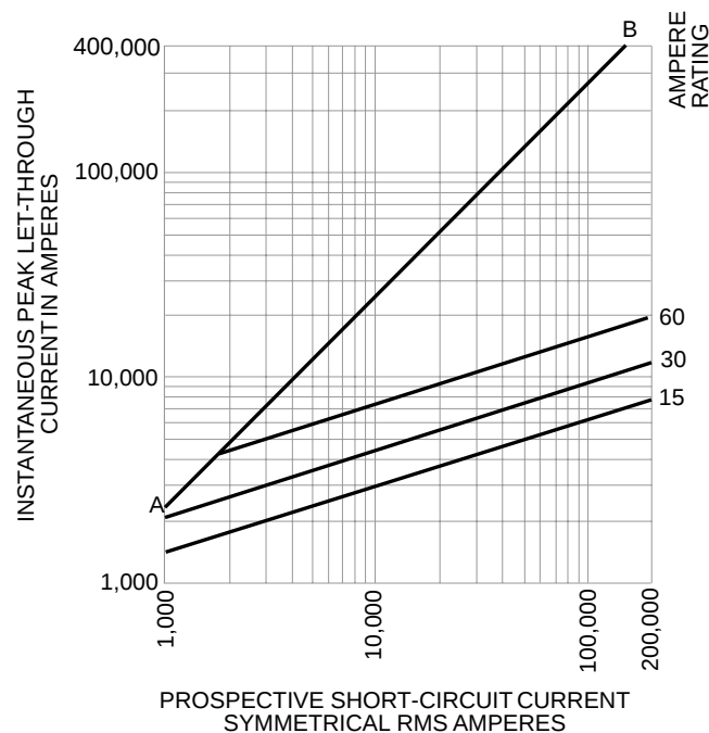
Current-Limitation Curves
