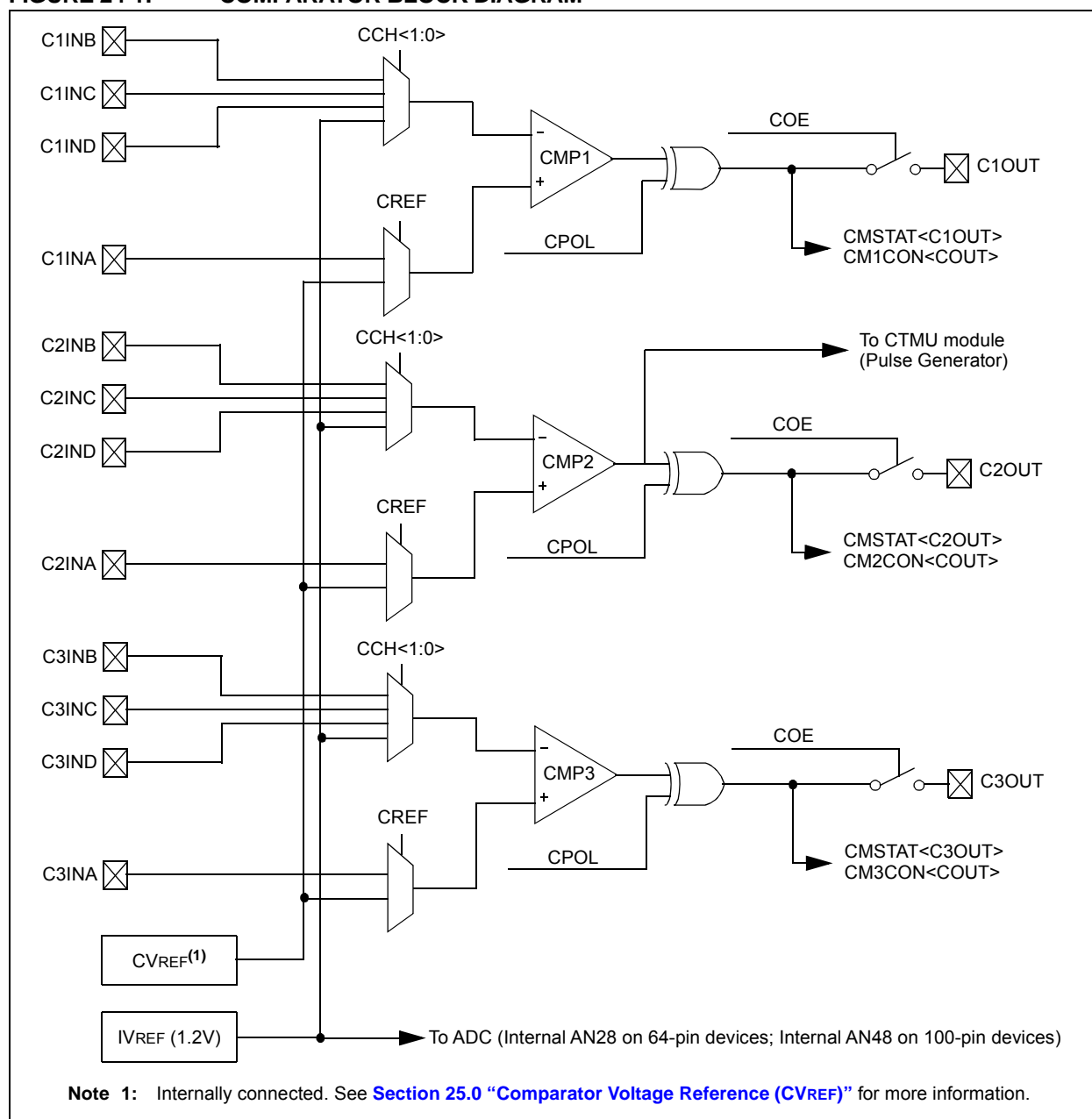
FIGURE 24-1: COMPARATOR BLOCK DIAGRAM
