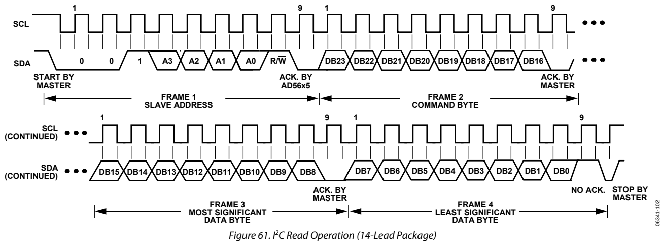
Figure 61. I²C Read Operation (14-Lead Package)
