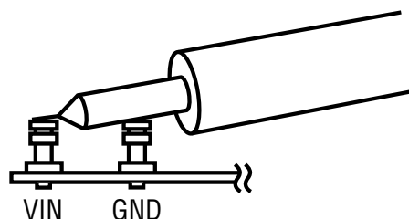
Figure 4. Measuring Input or Output Ripple
