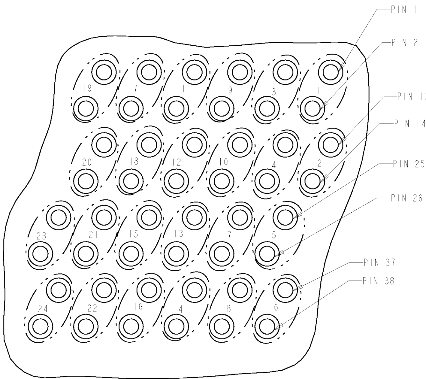
PRESS-FIT BOTTOM VIEW SCALE 4:1
